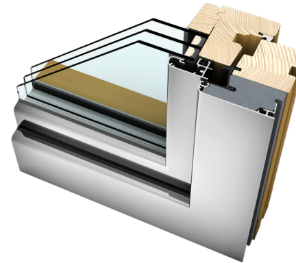
Cutaway of triple glazed aluclad timber window (Source: Internorm)
