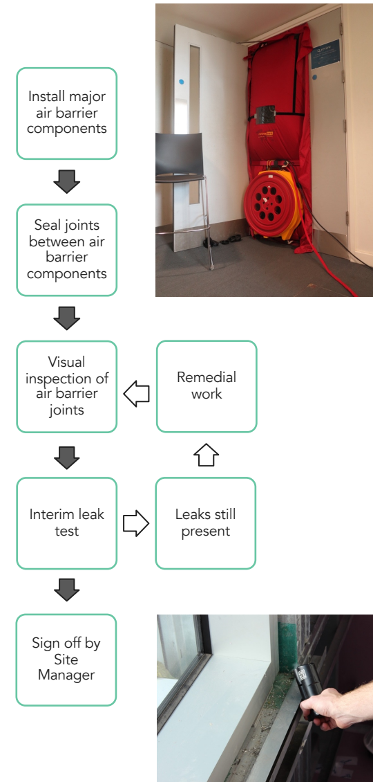
Recommended airtightness process: visual inspection, leak finding and interim air testing are all required before the final air test
