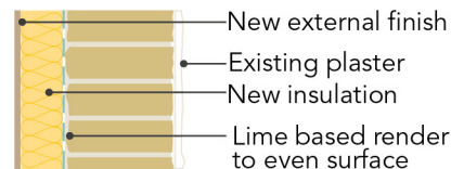
Externally insulated Stone Wall
