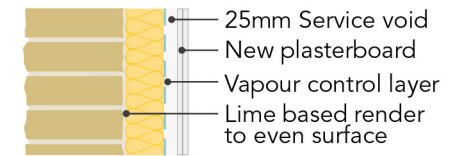
Internally insulated Stone Wall
